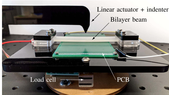
Fig. 8. Experimental setup for assessment of the mechanical performance, with the rigid base of the sensor replaced by a PCB, and a linear actuator equipped with an indenter to press on the sensor. The sensor and PCB are attached on a base that is mounted on a load cell to have ground truth force magnitude measurements.
