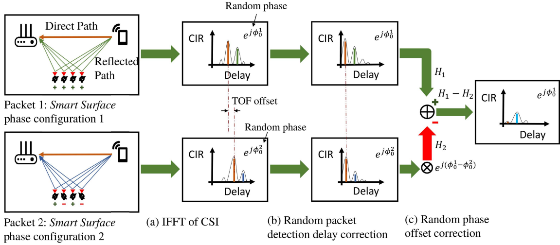
Figure 5: Illustration of ScatterMIMO's algorithm to compensate for packet detection delay and carrier phase offset using 1D IFFT.
